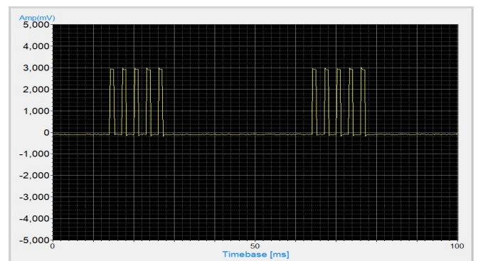
Multiple pulse signal (Pulse signal generator)
