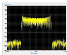
FM modulation Signal
