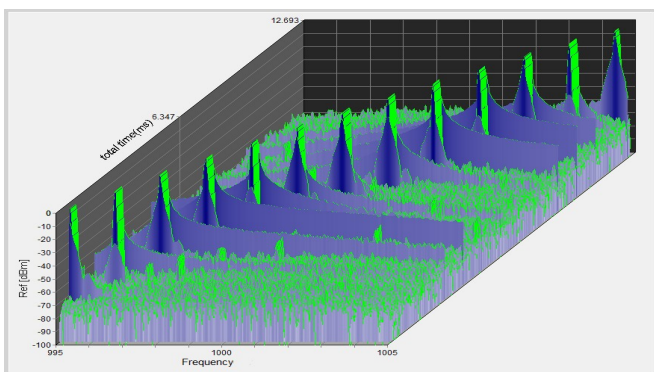
Linear frequency sweep (RF signal generator)
