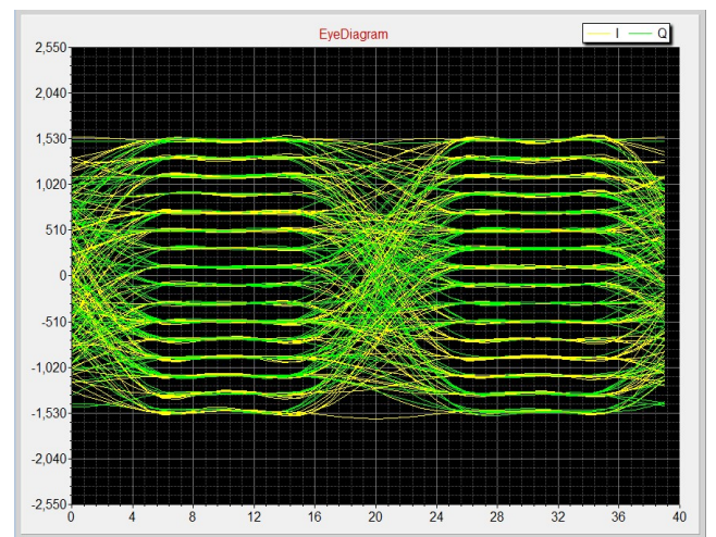
256-QAM eyes diagram
