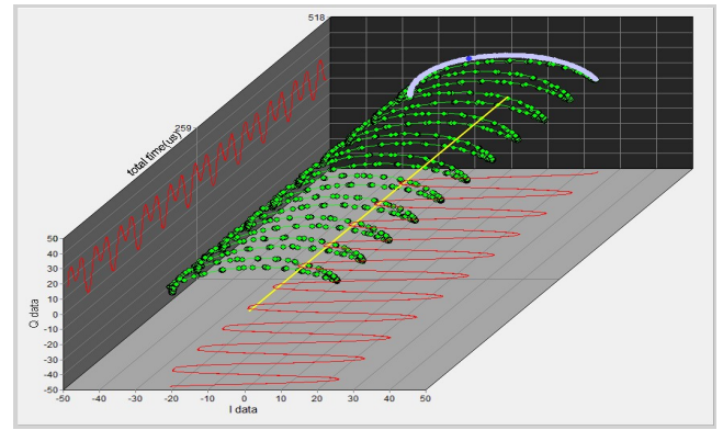
3D PM Signal (STFT phase)
