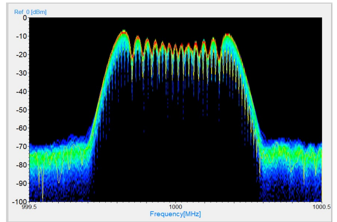
FM modulation
