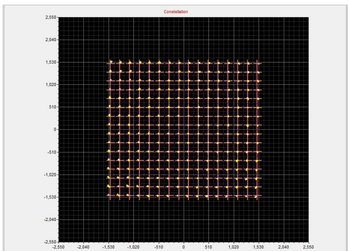
256-QAM Constellation
