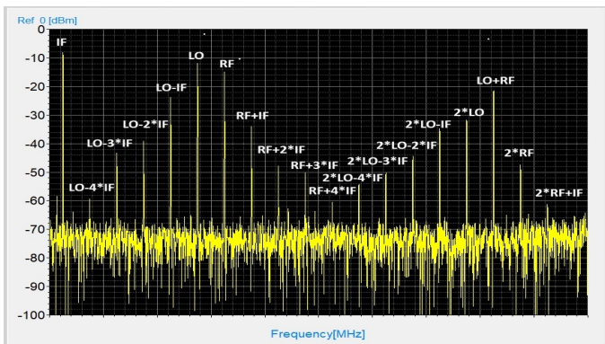
Hopping Sweep Mode
