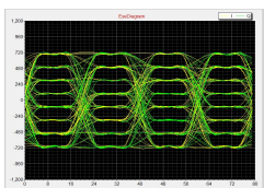
64 QAM eyes diagram
