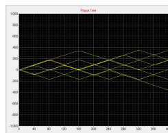
MSK Phase tree
