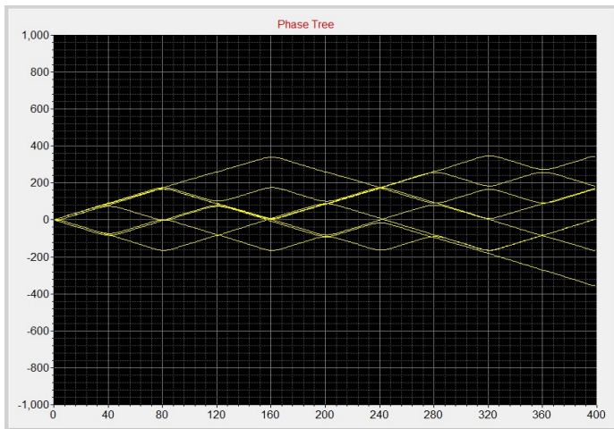
MSK phase tree
